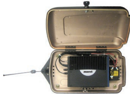
Inside of Enclosure for M5300 and XG-75M Motorcycle Kit
